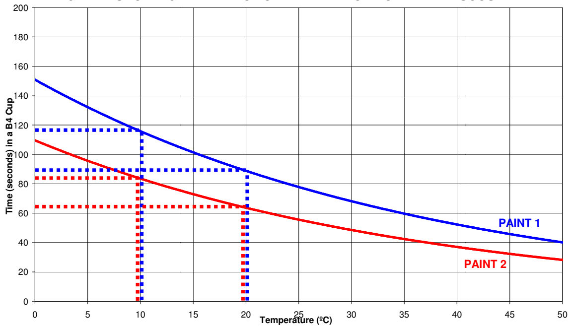
GRAPH SHOWING THE EFFECT OF TEMPERATURE ON PAINT VISCOSITY
